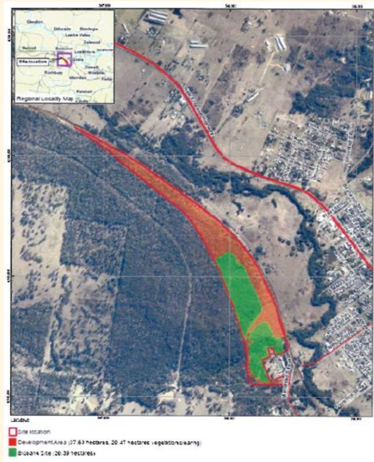
Figure 1: Proposed GTSF
