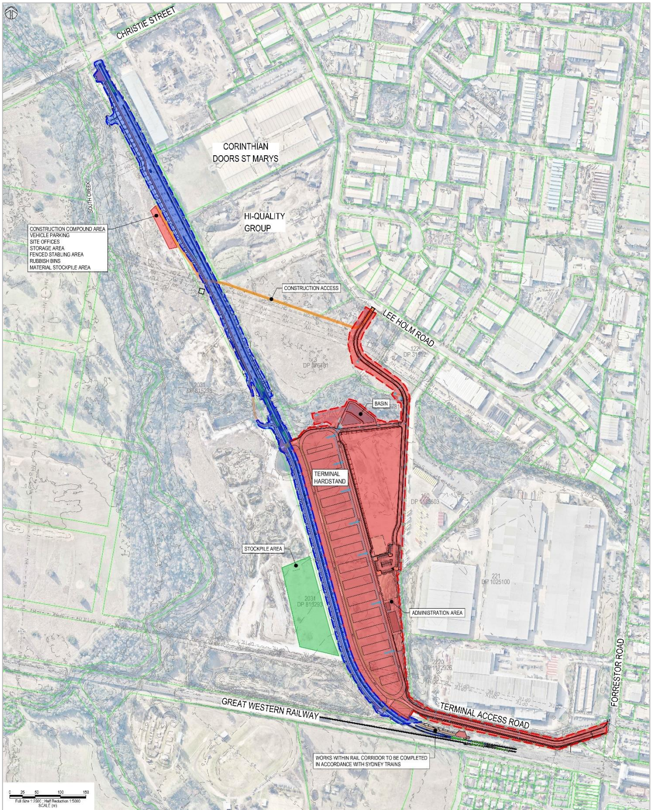
Figure 1: General Site Plan (as modified)
